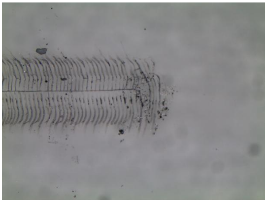
Hard Coating with 9H Pencil Test
